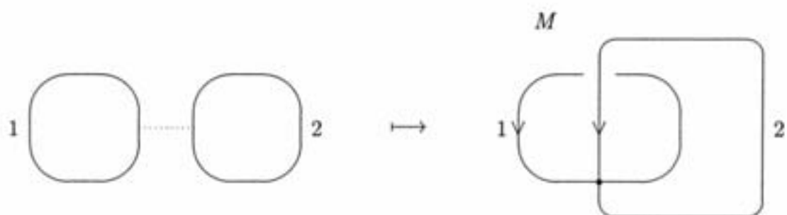
Figure 4: A chord diagram on M .
