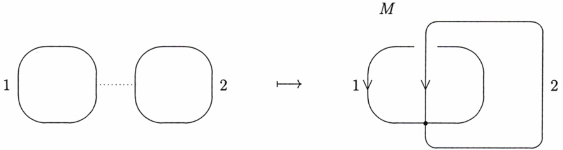
Figure 4: A chord diagram on M .
