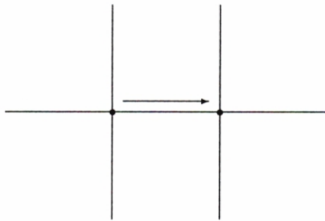
Figure 5: Approaching a boundary on \text{ch}(M) .
